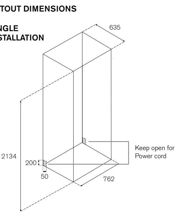
SIDE BY SIDE INSTALLATION
